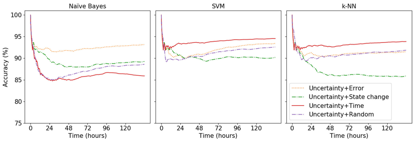
Fig. 8 The accumulated accuracy over time for the hybrid interactive learning strategies on the Occupancy dataset
