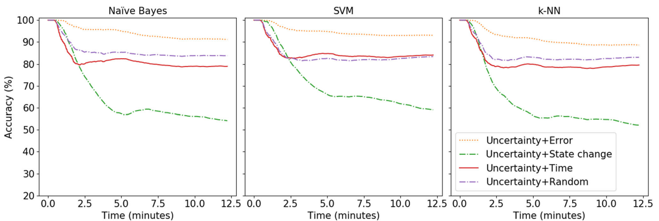
Fig. 7 The accumulated accuracy over time for the hybrid interactive learning strategies on the Opportunity dataset
